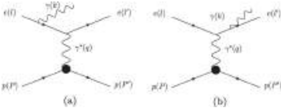
FIG. 7. The Bethe-Heitler process ep \rightarrow ep\gamma diagrams for (a) a photon emitted from an incident electron (preradiation) and for (b) a photon emitted from a scattered electron (postradiation).
