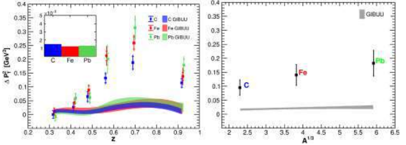
FIG. 4. Left (right): the z (nuclear radius)-dependent \Delta p_T^2 results for the three nuclei (results are horizontally shifted for clarity). The outer error bars are the p_T systematic uncertainties added in quadrature with the statistical uncertainties, while the normalization uncertainties are presented in the inset for the z dependence and found to be less than 1% for the A dependence. The GiBUU model calculations are represented by the colored (left) and shaded (right) bands obtained by interpolating the model points and their statistical uncertainties.
