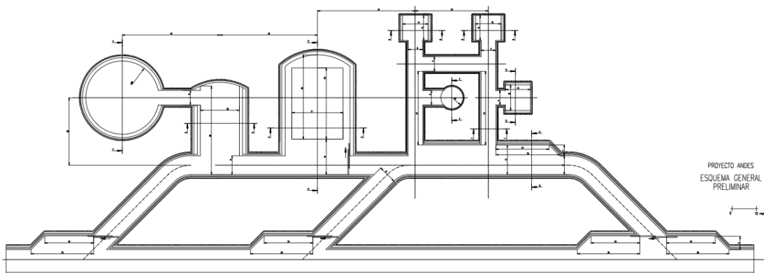
Fig. 5: Top view (not to scale) of the proposed underground site in its current preliminary status. Vehicle transit is from right to left.
