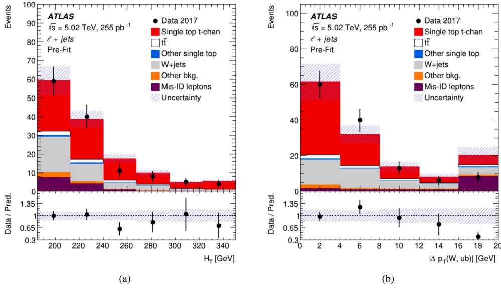
Fig. 2. The pre-fit (a) H_T and (b) |\Delta p_T(W, ub)| distributions for data (dots) in the inclusive \ell + \text{jets} channel. The MC simulation of the signal (red histograms) and various backgrounds (represented by histograms of different colours) are also included. The error bars on the dots represent the statistical uncertainty on the data while the blue cross-hatched lines correspond to the total uncertainties on the prediction. The lower panels show the ratio of the data and the prediction, along with the uncertainty in the ratio. The last bin includes any event overflows. The \chi^2/\text{degrees of freedom} are evaluated to be 2.5/6 for (a) and 5.9/5 for (b).
