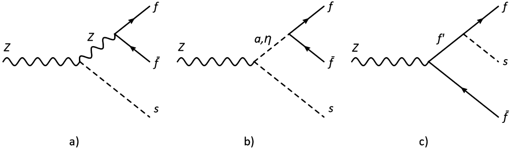
Fig. 3. Feynman diagrams corresponding to the Z \rightarrow s^0 f \bar{f} : a) exchange of virtual Z , b) exchange of virtual a and \eta and c) exchange of virtual fermion f' .
