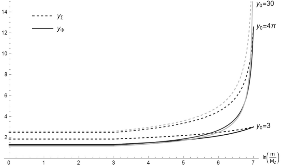
Fig. 2. A solution for y_\Sigma and y_\Phi of the RGEs for the boundary conditions (35) given by three values y_0 = 3, 4\pi, 30 , and for \Lambda = e^7 M_Z \approx 100 \text{ TeV} and M_R = e^3 M_Z \approx 1.8 \text{ TeV} .
