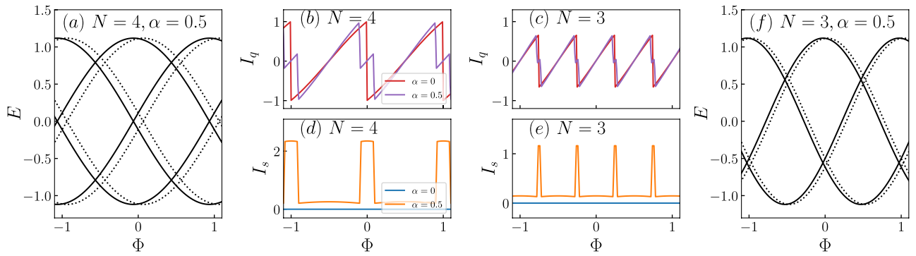
Figure 4. Quasiparticle spectra and corresponding charge and spin persistent currents, I_q and I_s respectively, for \lambda_1 = \lambda_2 = \xi_M = 0 . The number of sites, N , and the Rashba spin-orbit coupling, \alpha , are indicated in the figures.
