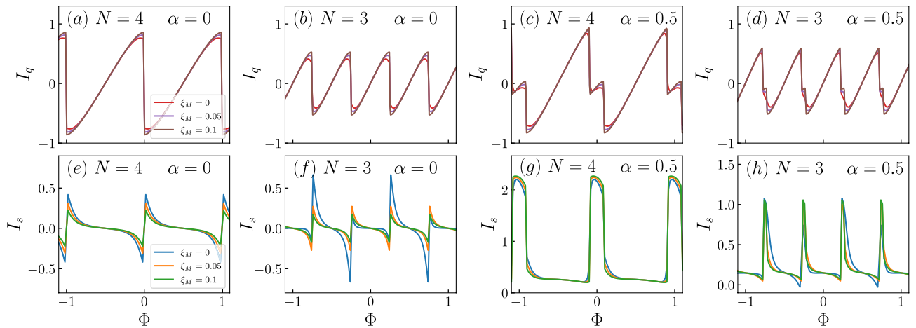
Figure 5. Charge and spin persistent currents, I_q and I_s respectively, for \lambda_1 = 0.1, \lambda_2 = 0 . The number of sites, N , and the Rashba spin-orbit coupling, \alpha , are indicated in the figures. The coupling between MZMs, \xi_M , is indicated by coloured lines, shown in the leftmost panels.
