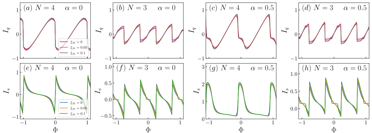
Figure 6. Charge and spin persistent currents, I_q and I_s respectively, for \lambda_1 = 0.1, \lambda_2 = 0.15 . The number of sites, N , and the Rashba spin-orbit coupling, \alpha , are indicated in the figures. The coupling between MZMs, \xi_M , is indicated by coloured lines, shown in the leftmost panels.
