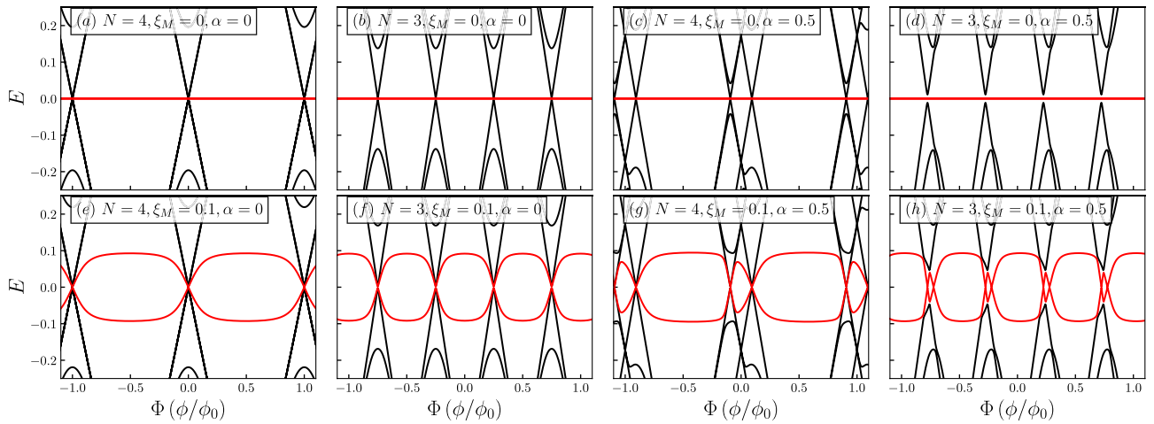
Figure 2. Quasiparticle spectra for \lambda_1 = 0.1 and \lambda_2 = 0 . The number of sites, N , the coupling between MZMs, \xi_M , and the Rashba spin-orbit coupling, \alpha , are indicated in the figure. Black curves represent the states in the quantum ring and the red curves correspond to the Majorana modes.
