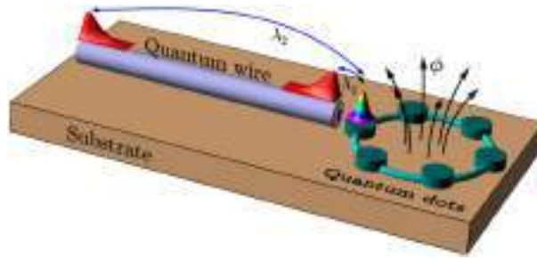
Figure 1. (a) Schematic representation of the system under study. A nanowire driven into a superconducting regime supports a MZM at each edge and influences the persistent currents of a quantum ring, threaded by a magnetic flux. (b) The quantum ring consists of an array of quantum dots uniformly distributed on a circumference. The MZMs are assumed to be coupled to the same quantum dot of the ring, with coupling constants \lambda_1 and \lambda_2 .
