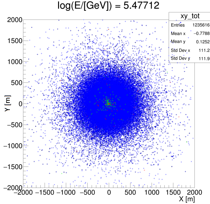
Figure 27: Footprint of an electromagnetic shower produced by a \gamma -ray of energy E_0 = 300 TeV, azimuthal angle \phi = 0 , and inclination \theta = 8 degrees. In green (red) electrons (positrons). Note that although this gamma ray collided the atmosphere with an inclination, the development of the shower is symmetrical respect to the vertical axis.
