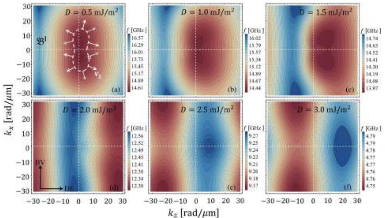
Figure 6. (a–f) Shows the isofrequency contours of band \mathcal{B}^I projected in the plane of the wave-vector space for different values of D . In (a), the directions of the group velocity vector are illustrated along a given slowness surface.
