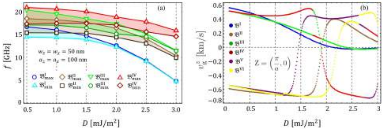
Figure 4. (a) Minimum and maximum values of the magnonic bands ( \mathfrak{B}_{\min}^n and \mathfrak{B}_{\max}^n ) as a function of the DM constant D . (b) z -direction component of the group velocity for the first 6 low-frequency bands at the Z point of the reduced Brillouin zone (DE configuration).
