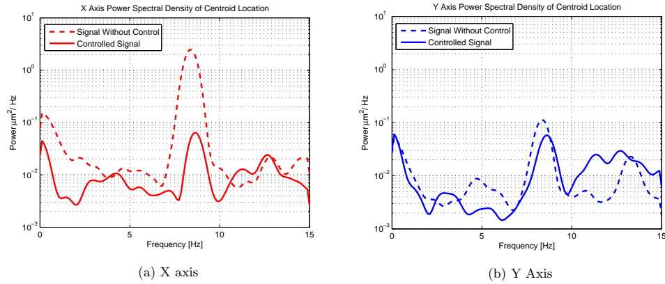
Figure 5: Closed Loop performance
