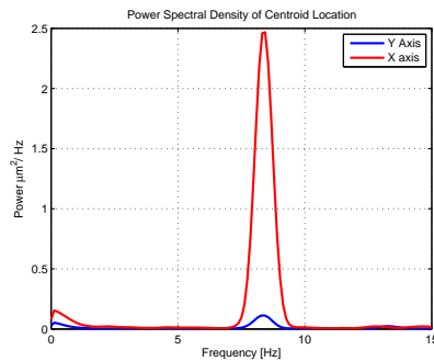
Figure 3: Power Spectral Density of the centroid movement without control in both axes
