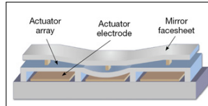
Figura 2.11: Espejo deformable MEMS
