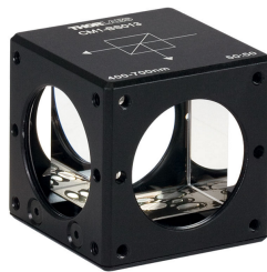
Figura 3.3: Beam Splitter CM1-BS013
