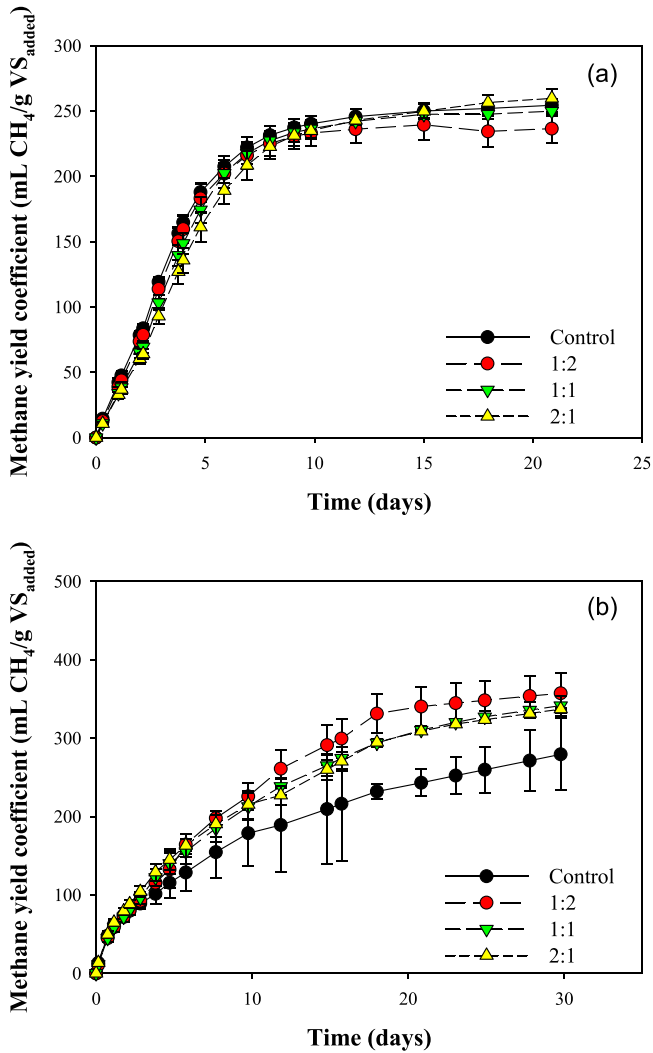
Fig. 2. Variation of the methane yield coefficient (mL CH 4 /g VS added ) for the control (no bulking-agent) and the assessed bulking-agent to substrate ratios for a) bean peel and b) food waste, throughout the experimental time; were VS, volatile solids.
