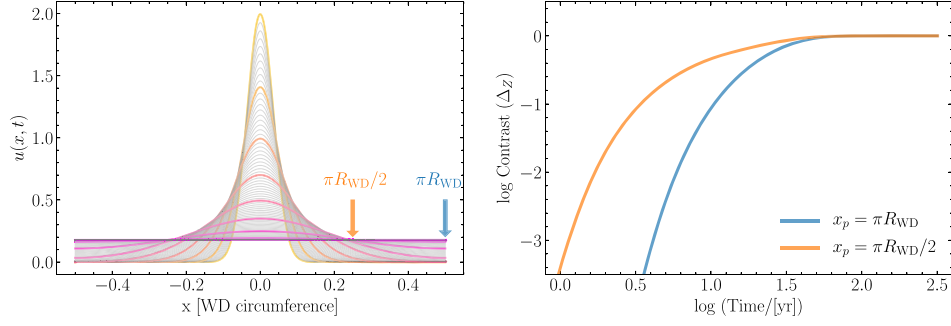
Figure 2. Left: Evolution of a passive scalar, u , according to equation (8) with a horizontal diffusion coefficient ( D_{\text{surf}} ) of 2 \times 10^9 \text{ cm}^2 \text{ s}^{-1} , characteristic of a white dwarf with T_{\text{eff}} = 12\,000 \text{ K} and \log g = 8.0 , and a typical white dwarf radius ( R_{\text{WD}} ) of 0.012\,88 R_{\odot} . To make clear the evolution, every 10th (logarithmic) time-step is indicated with a colour: from yellow to purple. Right: Examination of the time-dependent contrast between points of interest along the white dwarf circumference. Here, we define contrast ( \Delta z ) according to equation (13) and show the evolution of \Delta z at half and a quarter of the circumference.
