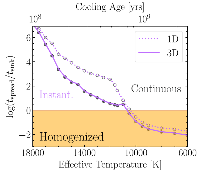
Figure 10. Comparison of two models, instantaneous accretion (purple lines) and continuous accretion (grey circles), in the comparison of spreading and sinking time-scales for H-rich atmospheres at \log g = 8.0 . The instantaneous accretion model is shown where the vertical sinking velocity, v_{\text{drift}} , is either given by the 1D mixing length theory results of Koester et al. (2020) or from the 3D overshoot results of CU19 (see Fig. 9) in dotted or solid, respectively. The spreading time-scale is defined for a maximum surface abundance contrast of \Delta_Z = 0.37 from equatorial accretion (reproduced from lower panel; Fig. 8). The latter model – continuous accretion – is expressed by the left-hand side of equation (19) as a mean across the elements O, Mg, Si, Ca, and Fe. The overshoot and no overshoot description of the continuous accretion case is indicated by filled and open circles, respectively.
