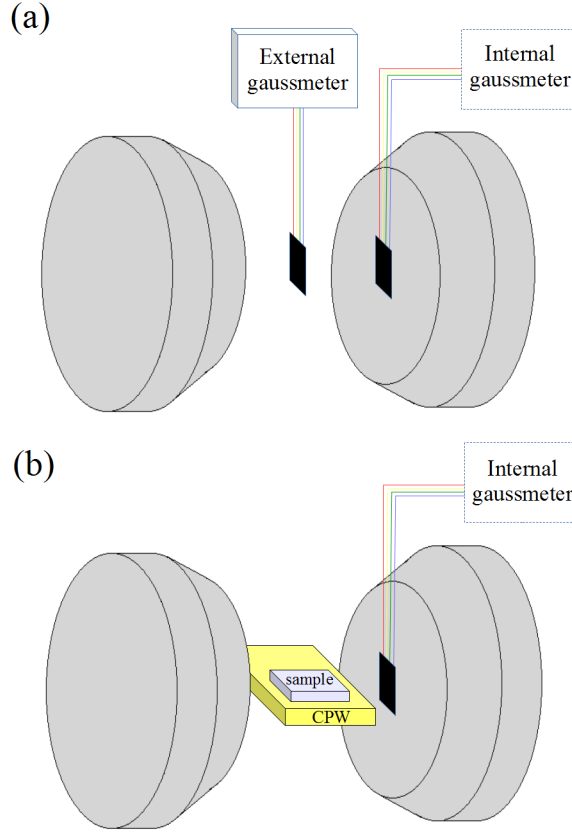
Figure 3.4: Magnetic field calibration steps: (a) An external Hall effect sensor is placed in the gap between the magnet poles and its readings are correlated with another permanently attached to one of the poles, (b) During measurements the value of H felt by the sample is interpolated by the reading of the fixed Hall effect sensor.
