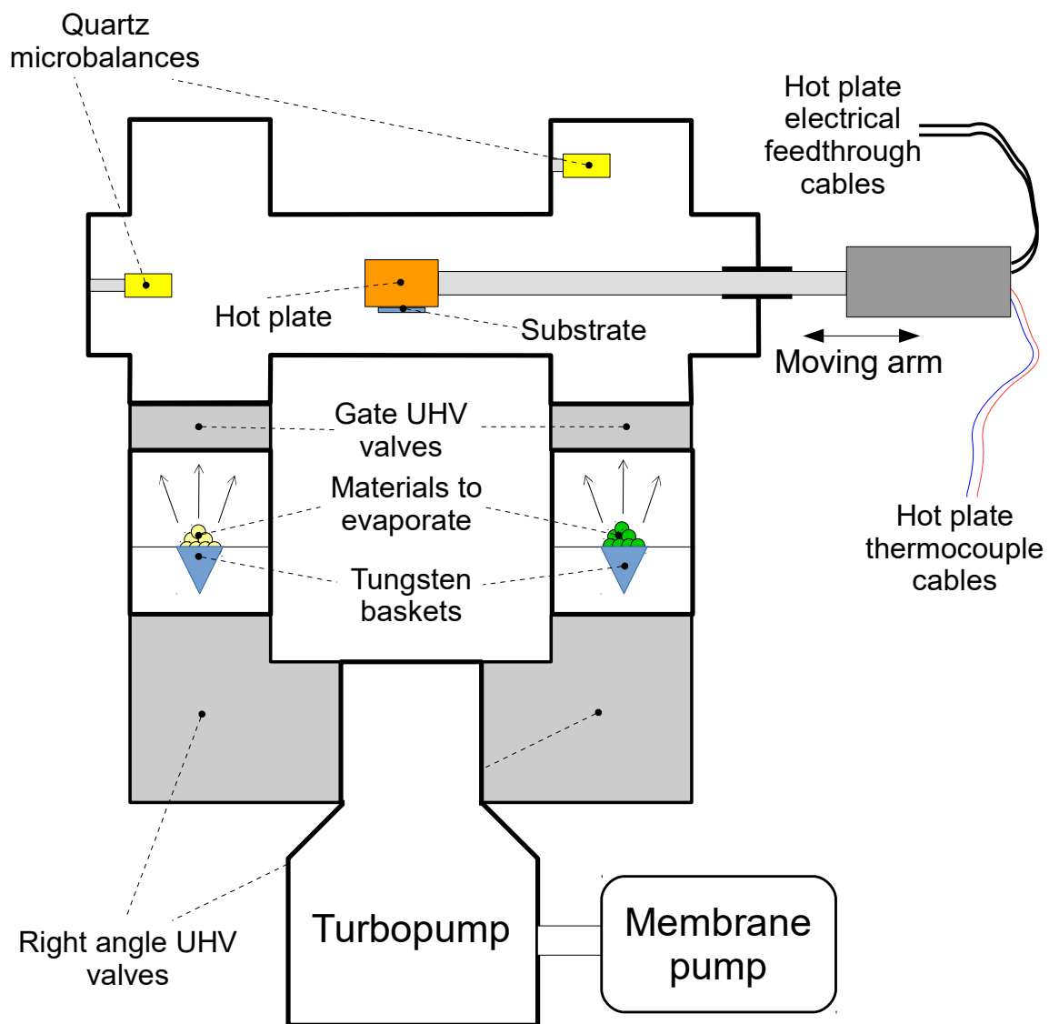
Figure C.1: Sketch of the 2-material thermal evaporation chamber built during my thesis.
