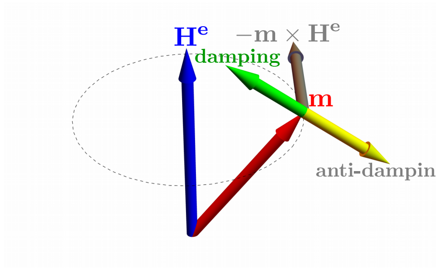
Figure 1.2: Effect of the anti-damping force on the precision of \mathbf{m} .
