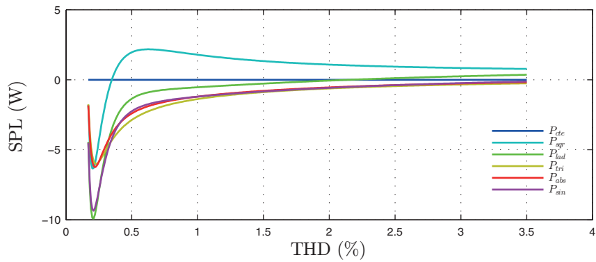
Figure 5.24: Switching losses for each pondering profile compared to a constant pondering profile
