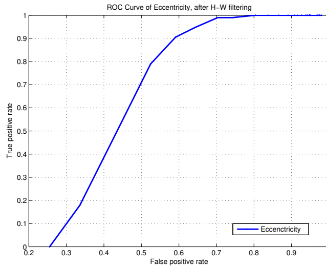
Figure 4.6. ROC curve of size features, after filter by bounding box.
