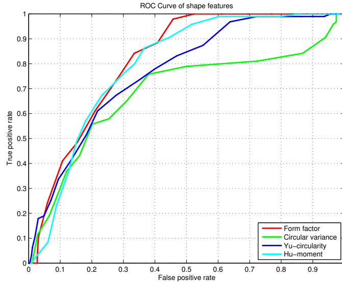
Figure 4.8. ROC curve of shape features.
