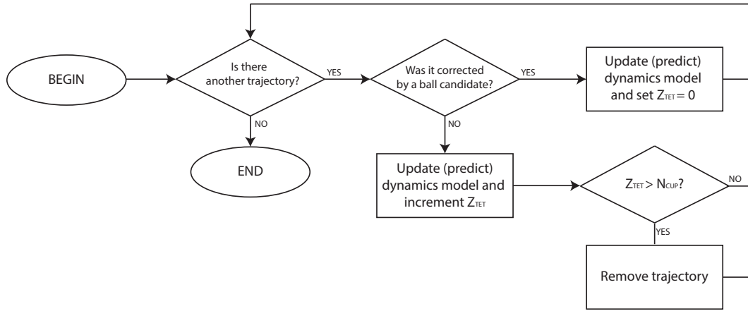
Figure 5.3. Flowchart of the trajectory update process.
