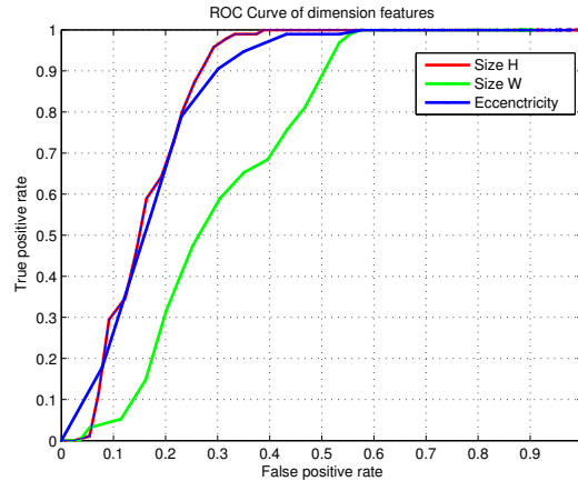
Figure 4.5. ROC curve of size features.
