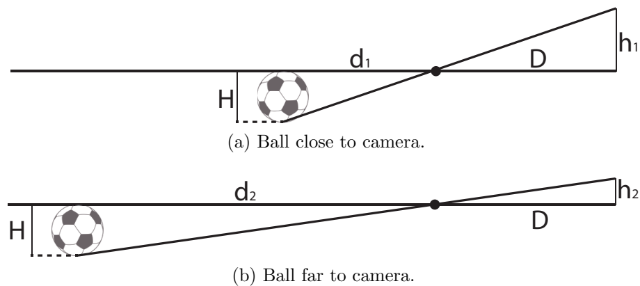
Figure 4.1. Pinhole principle.
