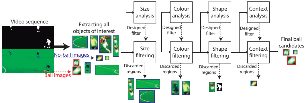
Figure 4.4. Preliminary tests to design coarse-to-fine structure.
