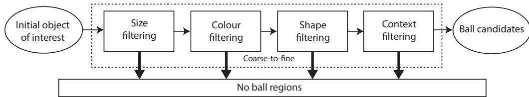
Figure 4.3. Coarse-to-fine structure for detecting ball candidates.
