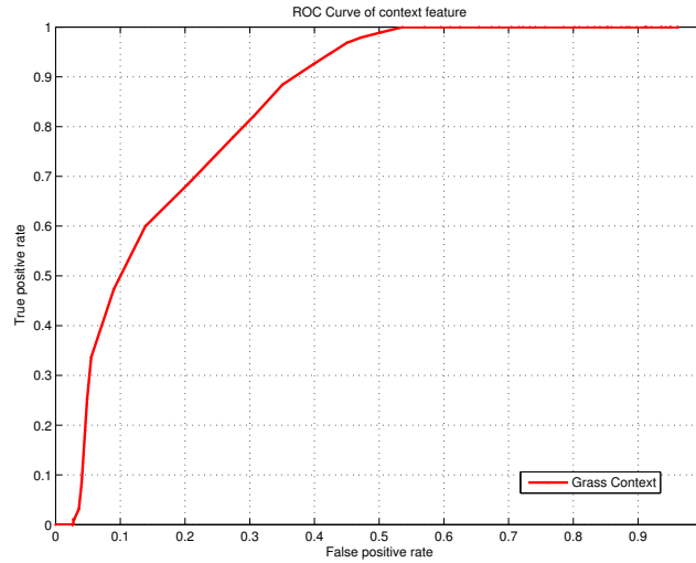
Figure 4.10. ROC curve of context feature.
