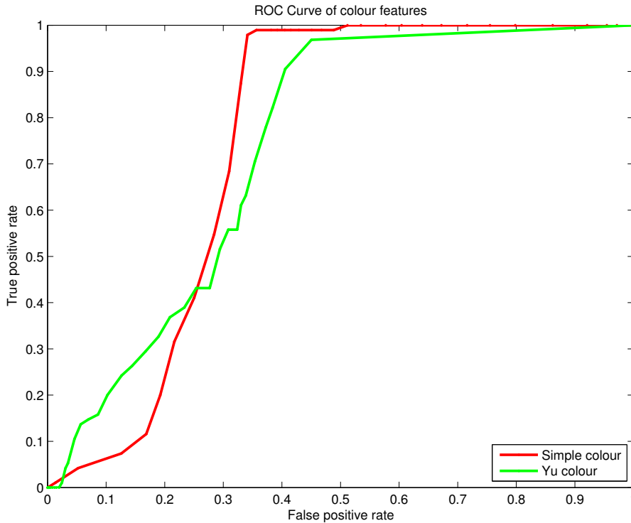
Figure 4.7. ROC curve of colour features.
