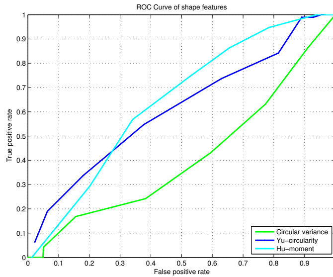
Figure 4.9. ROC curve of shape features, after filtering by form factor.
