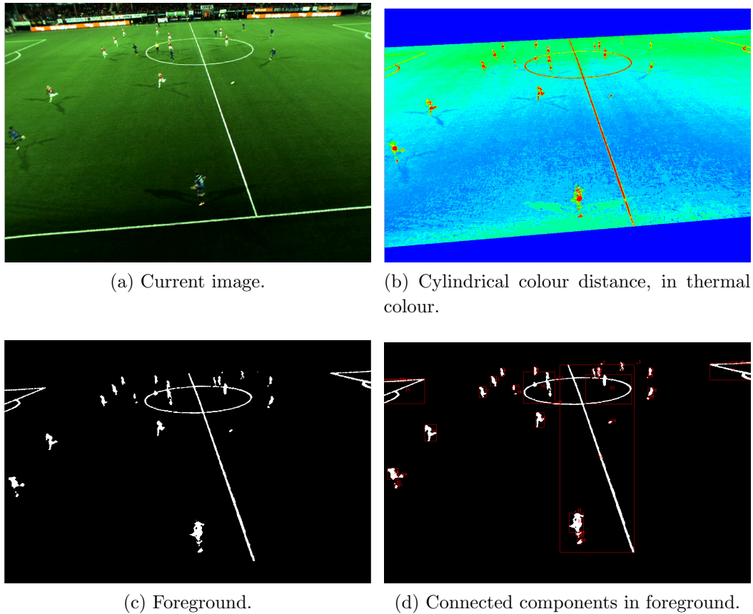
Figure 3.3. Segmentation process.
