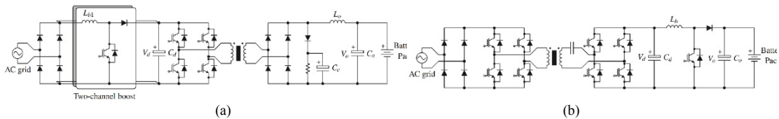
Fig. 3. Examples of two-stage on-board chargers with HF galvanic isolation and dedicated charging converter. (a) Full-bridge converter with interleaved boost PFC. (b) Uncontrolled LLC resonant converter with low-voltage boost PFC.
