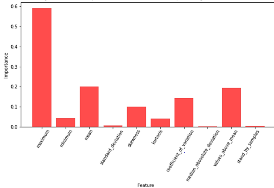
(b) Feature importance selecting all features for the best configuration parameters in Dataport.
