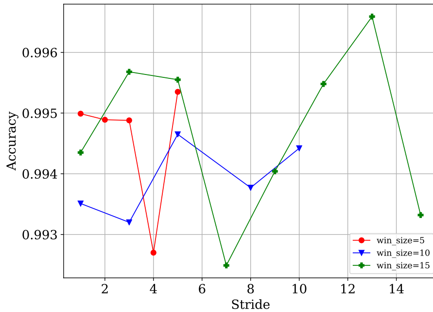
(a) Accuracy obtained for different values of stride and window size with Dataport data.
