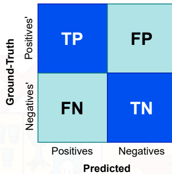
Figure 2.3: Confusion matrix representation.
