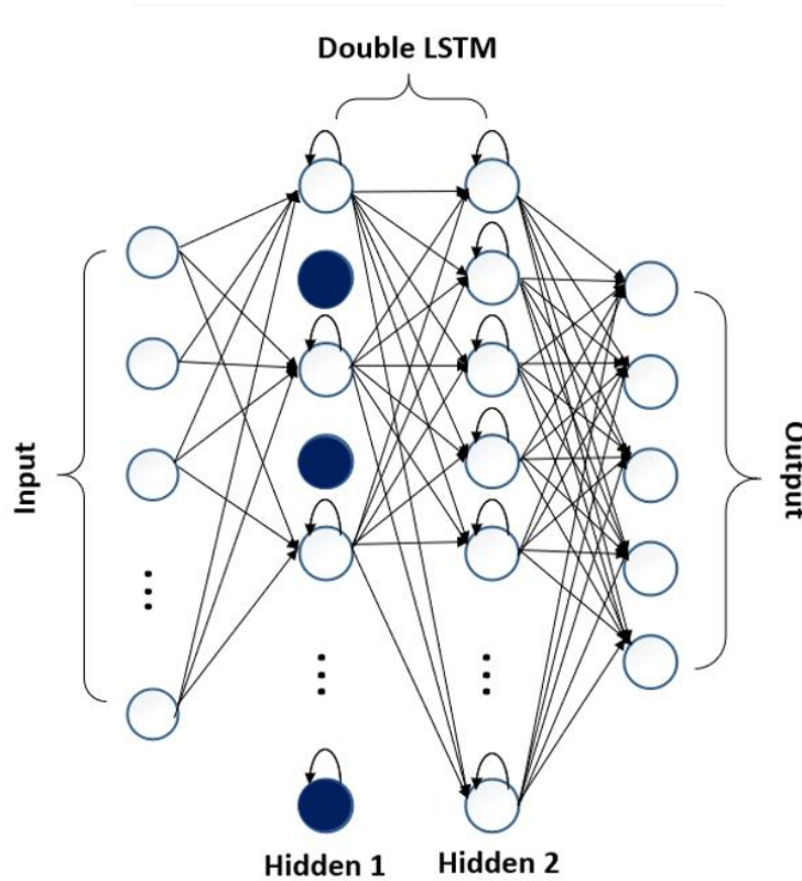
Figure 3.4: Proposed LSTM classifier architecture. The model has 10 input neurons, a double LSTM hidden layer of 200 cells each. Dropout has been set for the first hidden layer with 0.5 probability. The off neurons have been represented in dark blue.
