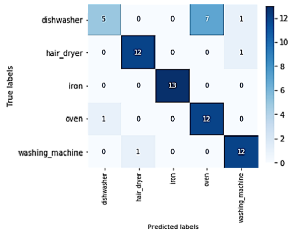
(c) Confusion matrix SVM classifier.
