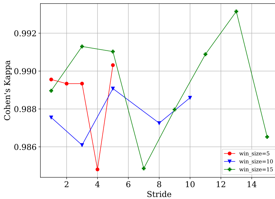
(b) Cohen's Kappa coefficient obtained for different values of stride and window size with Dataport data.
