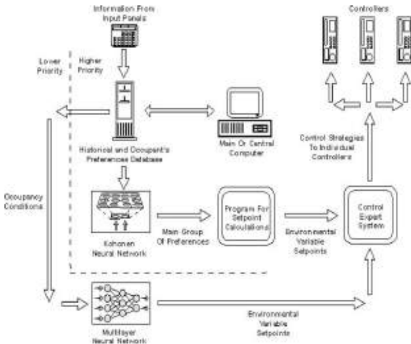
Fig.1. Intelligent System Architecture where the negotiating agent resides in main computer
