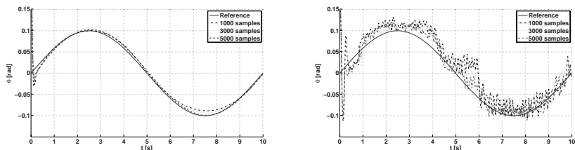
Fig. 5 Performance with \vartheta_{ref} sinusoidal (left:NN, right:Extra-Trees)
